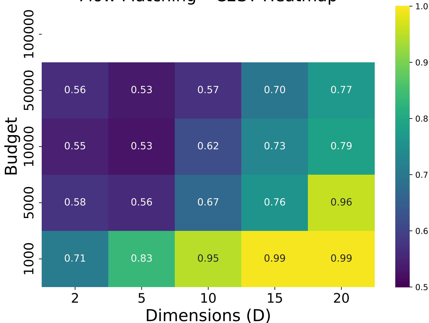
Flow Matching - C2ST Heatmap
